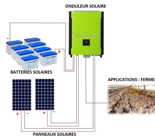
INSTALLATION AUTONOME
