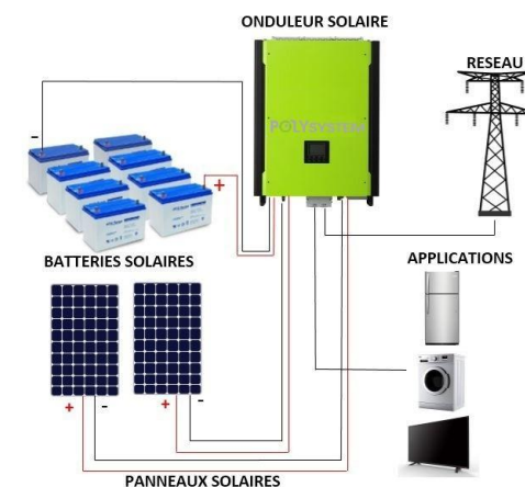
INSTALLATION HYBRIDE
