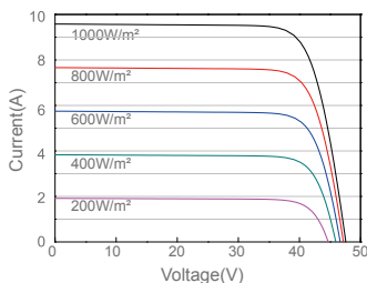
Current-Voltage Curve JAM72D00-355/PR
