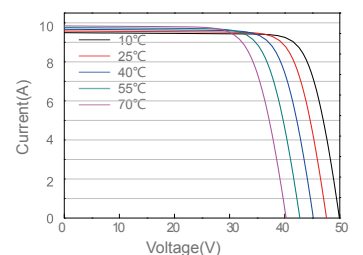
Current-Voltage Curve JAM72D00-355/PR
