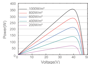
Power-Voltage Curve JAM72D00-355/PR
